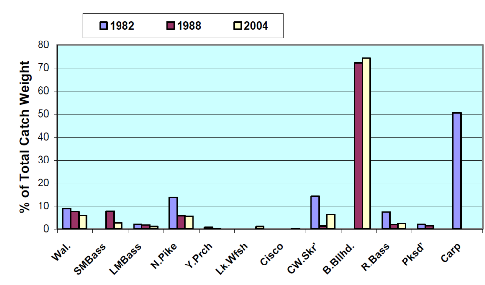
Figure 22. Catch composition by species for the 1982, 1988, and 2004 trapnet surveys on Manitowabing Lake (McIntyre, 2005).
