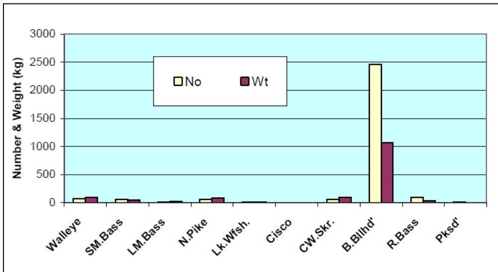
Figure 21. Catch composition for the 2004 ESTN survey on Manitowabing Lake (McIntyre, 2005).
